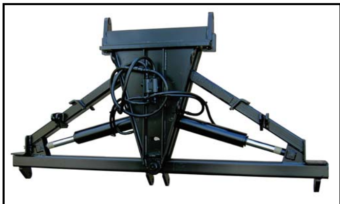
HD PRR DOUBLE RAM WITH CUSHION VALVE
